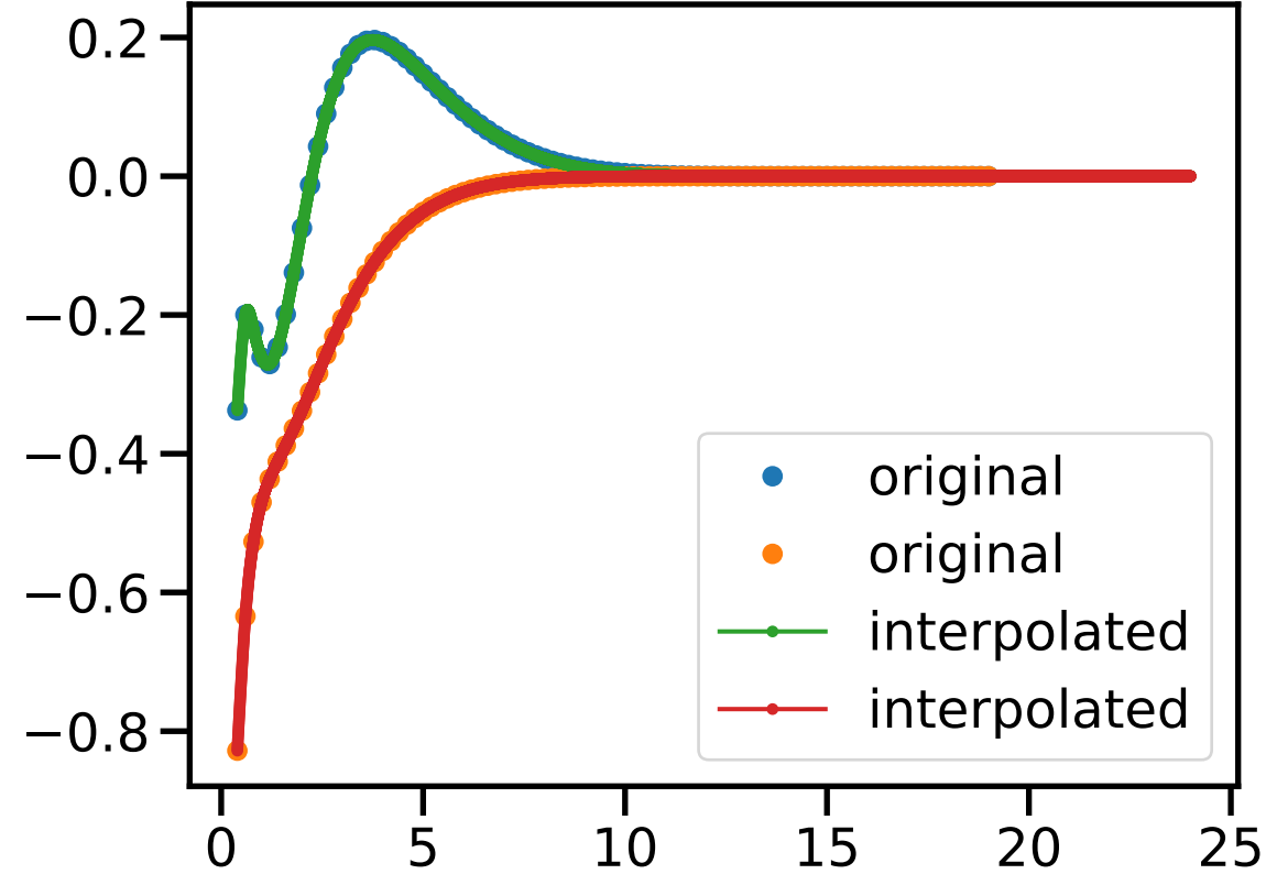
Hamiltonian Interpolation Before Training (14, 14, 1, 1)
